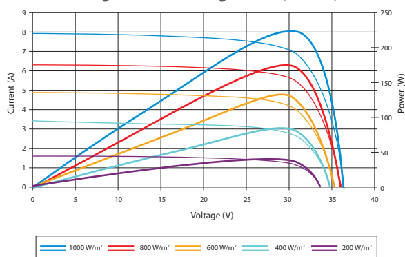
Current-Voltage & Power-Voltage Curve (225-20)
